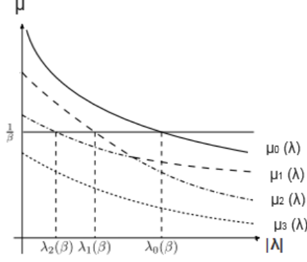
Figure 4.4: Graph of eigenvalues of \mu_j(\lambda) .
