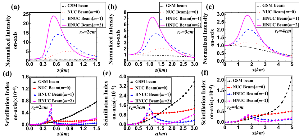
Fig. 5. Normalized intensity on-axis (a)–(c) and scintillation index on-axis (d)–(f) of HNUC beams propagation in turbulence with different beam order and different coherence length.
