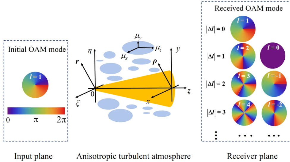
Fig. 2. Schematic diagram of the effects of an anisotropic turbulent atmosphere on the OAM mode.
