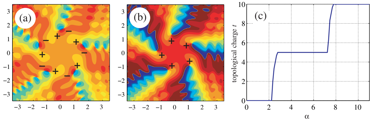
Fig. 6. Illustrating a jump of topological charge greater than 1 for m = 5 . (a) The case \alpha = 1.95 . (b) The case \alpha = 3.2 . (c) The topological charge as a function of \alpha .
