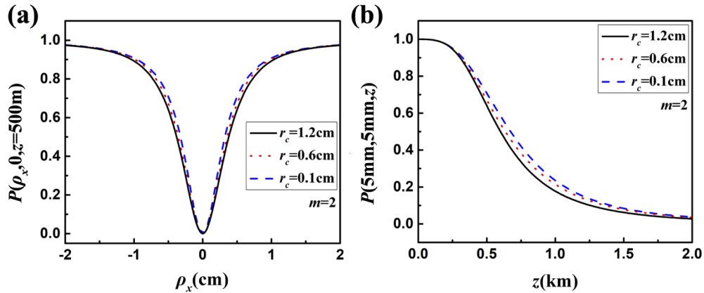
Fig. 6. DOP of RPHNUC beams (a) at z = 500\text{m} (cross line \rho_y = 0 ); (b) at point (5mm, 5mm) versus the propagation distance z in turbulence for different coherence width.
