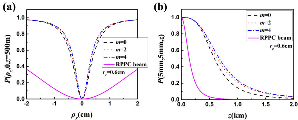
Fig. 5. DOP of RPHNUC beams (a) at z = 500\text{m} (cross line \rho_y = 0 ); (b) at point (5mm, 5mm) versus the propagation distance z in turbulence for different mode order.
