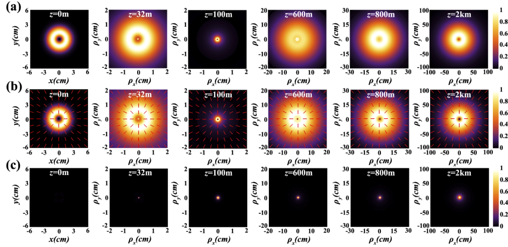
Fig. 3. Normalized intensity distributions of (a) RPHNUC beams, (b) its completely polarized part and (c) its completely unpolarized part with m = 1 on propagation in turbulence.
