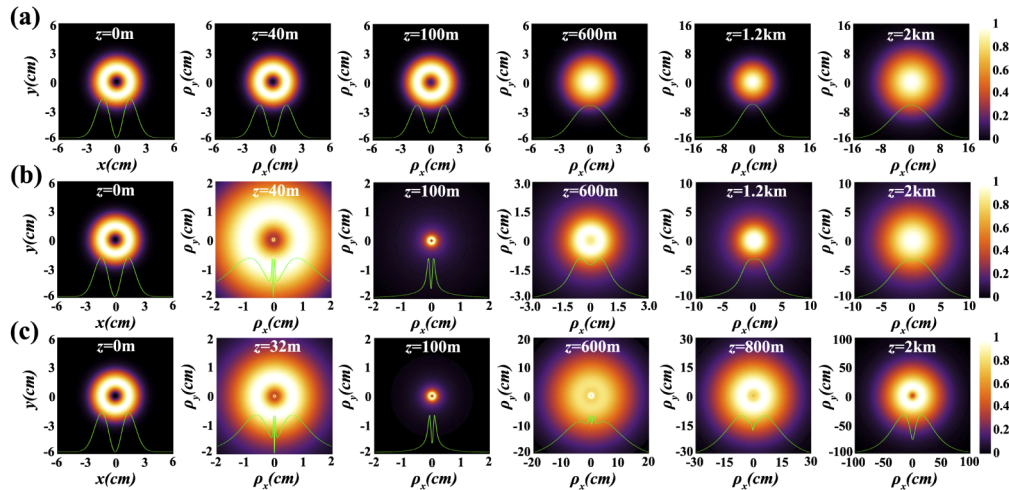
Fig. 1. Density plot of the normalized intensity of (a) RPPC beams and RPHNUC beams upon propagation in turbulence at different distances with different mode orders (b) m = 0 (c) m = 1 .
