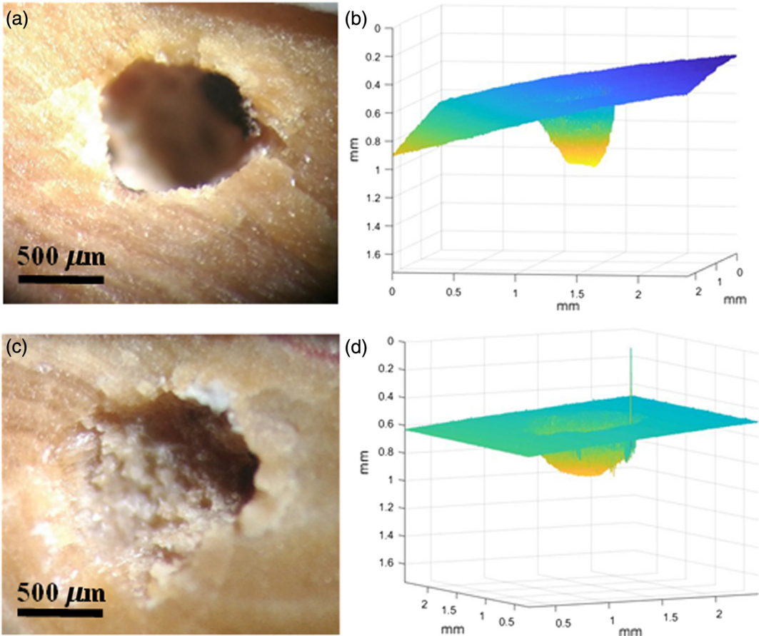
Fig. 8 Comparison between (a, b) fixed fiber and (c, d) vibrating fiber ablation for 150- \mu\text{m} -core fiber. Images (b, d) represent the OCT imaging reconstruction in MATLAB to determine cross-sectional area, volume, and axis length.
