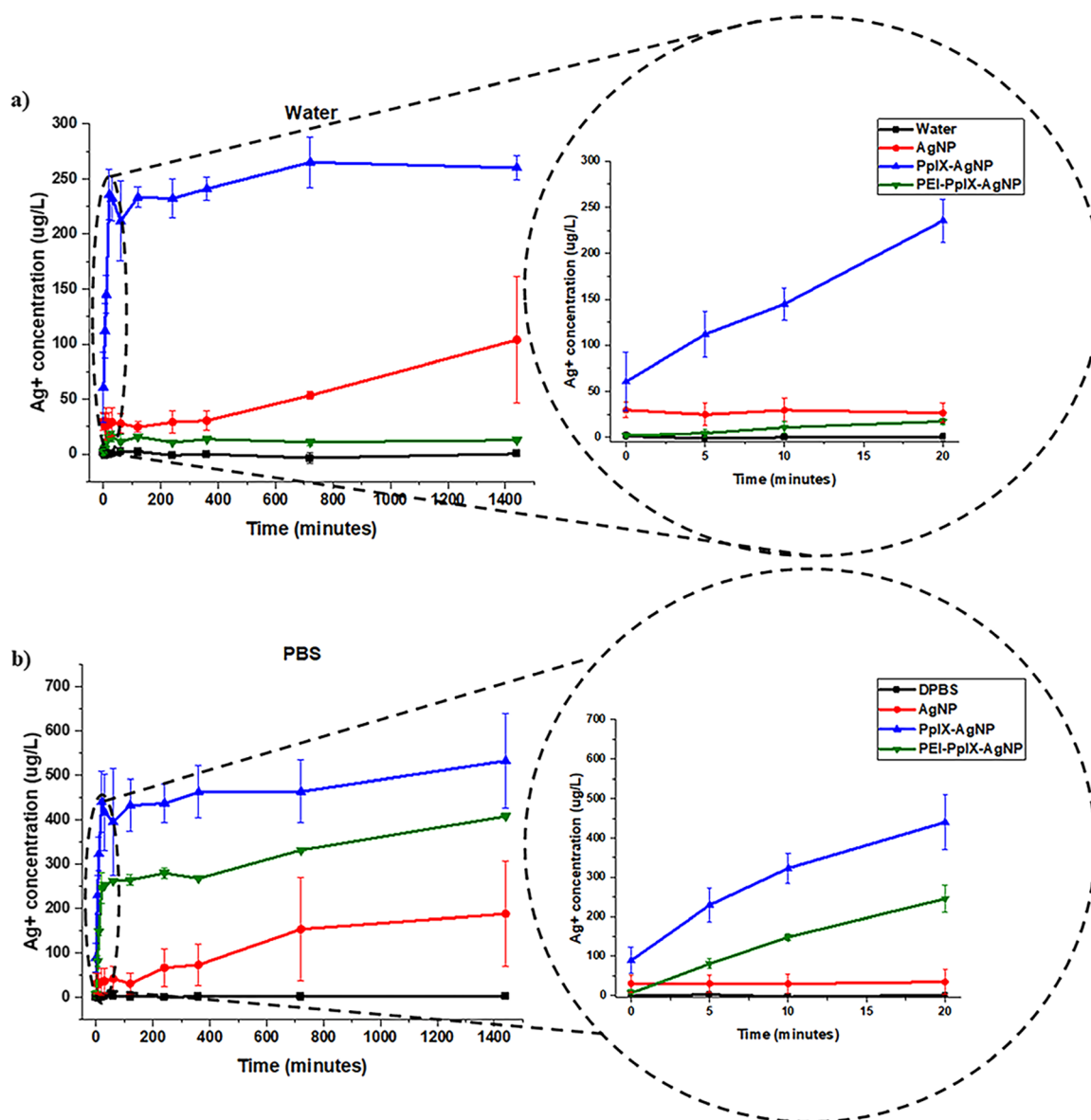
Fig. 2 \text{Ag}^+ release kinetics for AgNPs, PpIX-AgNPs and PEI-PpIX-AgNPs measured in (a) water or (b) DPBS. A zoom-in of the first 20 minutes are localized on the right.
