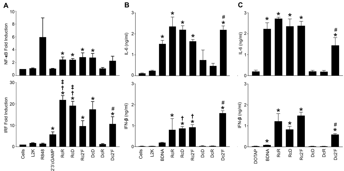
Figure 5. 2'F modified NANPs stimulate NF- \kappa B and IRF mediated cytokine production. (A) THP-1 Dual reporter cells were transfected with 5 nM NANPs for 24 h using L2K. Induction of the NF- \kappa B pathways was conducted using Quanti-Blue to monitor SEAP activity. Induction of the IRF pathway was conducted using Quanti-Luc to monitor the activity of secreted luciferase. (B, C) Microglia were transfected with 5 nM NANPs using either L2K (B) or DOTAP (C) for 4 h and cell supernatants were collected 24 h post transfection. Cell supernatants were then analyzed for cytokine production using specific capture ELISAs for IL-6 and IFN- \beta . Data are represented as the mean \pm (SEM) for a minimum of three independent experimental replicates. Asterisks indicate statistical significance compared to L2K, pound symbols indicate statistical significance compared to DcR, dagger symbols indicate statistical significance compared to Dc2'F, double dagger symbols indicate statistical significance compared to Rc2'F (Student's t -test, P -value < 0.05).
