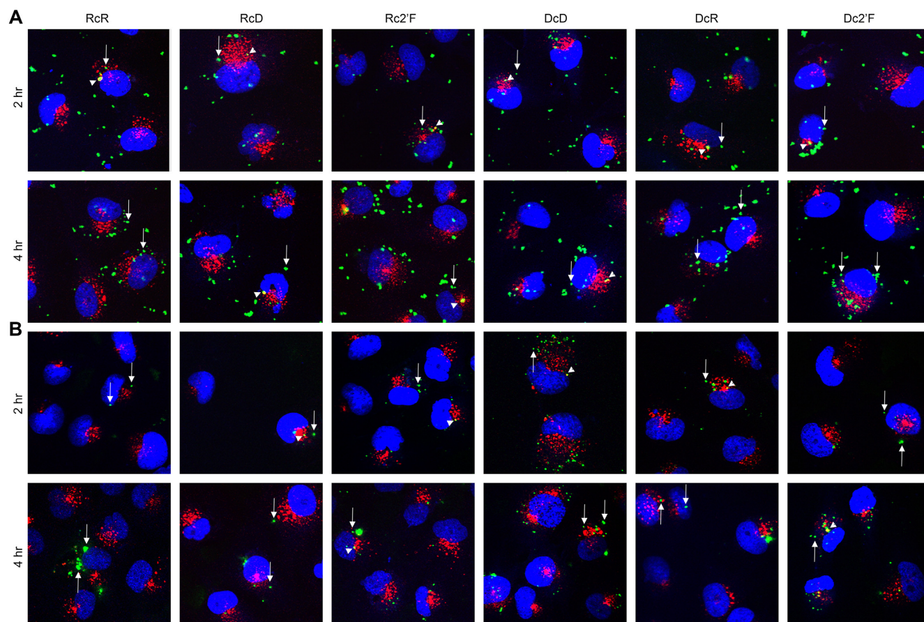
Figure 4. NANPs are internalized through endocytic pathway and traffic to the cytosol. Microglia were transfected with 5 nM Cy3-labeled NANPs using L2K (A) or DOTAP (B) for 2 or 4 h. Localization of NANPs (green) within cells was determined by immunofluorescence microscopy for the early endosomal marker, EEA1 (red), and nuclear stain DAPI (blue). Arrow heads indicate NANPs colocalized with EEA1, and arrows indicate NANPs that do not colocalize with EEA1.
