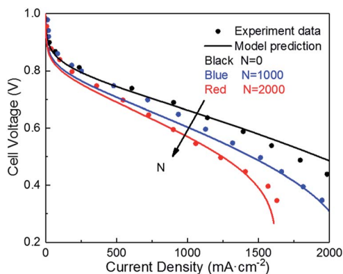
Fig. 4 Validation of polarization curve with experiments of ref. 9 during the potential cycling between 1 and 1.5 V_{\text{RHE}} with a sweep rate of 500 \text{ mV s}^{-1} (operating conditions: T = 80^\circ\text{C} , P = 1 atm, \text{RH} = 100\% ).
