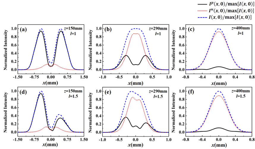
Fig. 4. Cross lines of the normalized intensity distributions I^p(x, 0)/\max[I(x, 0)] (solid black line), I^u(x, 0)/\max[I(x, 0)] (short dashed red line), I(x, 0)/\max[I(x, 0)] (long dashed blue line) of a focused partially coherent radially polarized vortex beam at several propagation distances for different values of topological charge l .
