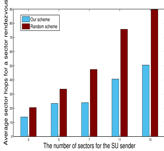
Figure 6.5: The average number of sector hops before a successful sector rendezvous.
