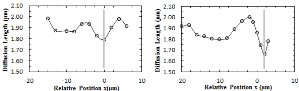
Figure 27: Plots of calculated diffusion lengths vs. distance from the defect center ( x = 0 \mu\text{m} on left, x = 2\mu\text{m} on right, indicated by vertical lines). The offset of the defect center on the right is a result of difficulty in positioning the sample with no visual reference for the defect.
