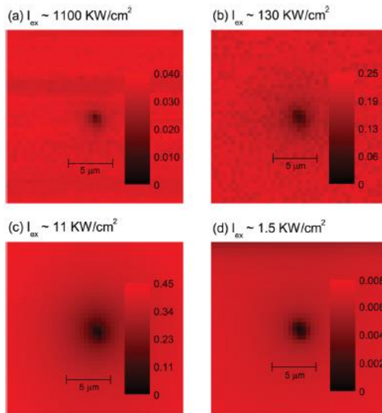
Figure 7: Plan view of confocal PL maps of an isolated dislocation in GaAs over a wide range of photoexcitation intensities I_{ex} ( I_{ex} values do not include reflection loss). Greyscale values are estimates of radiative efficiency- the ratio of photons emitted to photons absorbed (Gfroerer, Zhang, and Wanlass, 2013).
