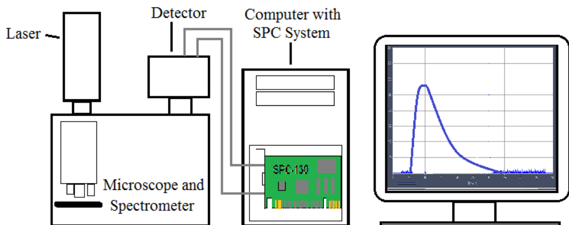
Figure 8: Block diagram of a typical TCSPC system connected to a confocal Raman/PL microscope. The display shows a nominal PL decay curve (a histogram made up of N time channels, where N can be 64, 256, 1024, or 4096 channels per curve). Adapted from the Becker and Hickl bh TCSPC Handbook , 6 th ed.
