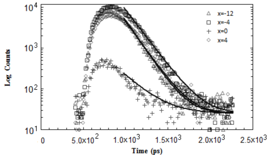
Figure 31: Semi-log plots of counts vs. time for four points near and in the defect. Solid lines represent attempts at nonlinear least squares fitting using MATLAB TM .
