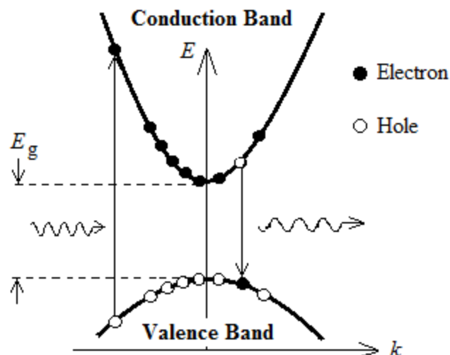
Figure 3: Photoluminescence in a direct bandgap solid. Absorption of photon with energy greater than E_g results in an electron being excited to the conduction band. Emission of a photon occurs as an electron in the conduction band falls to an available state in the valence band. Vertical transition arrows indicate momentum conservation (adapted from Fox, 2 nd Ed.).
