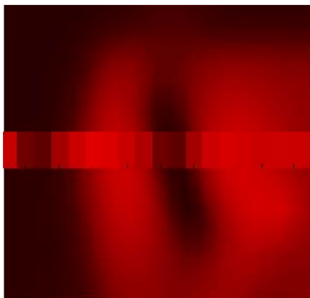
Figure 32: 1-D PL intensity map made with data from TCSPC system superimposed on 2-D PL map made using LabRam 800 Raman microscope. 1-D map data is taken from corrected total counts from figure 30.
