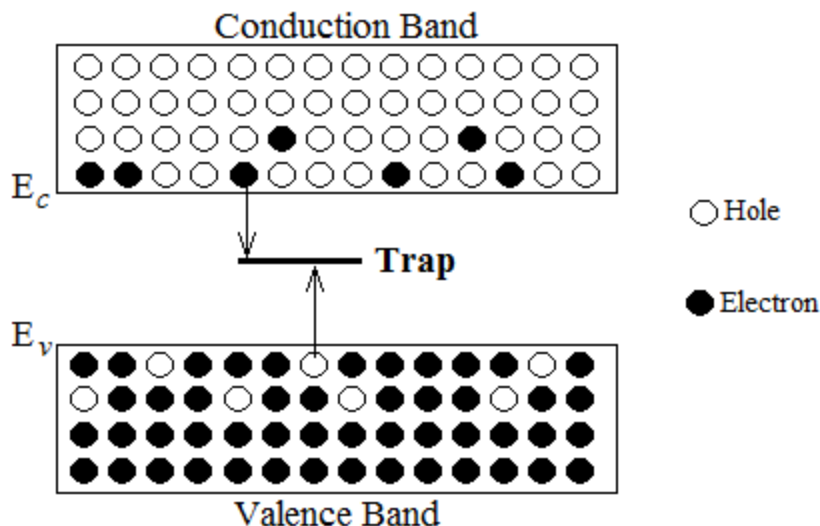
Figure 4: Electron-hole recombination via trap (adapted from Saleh and Teich, 2 nd Ed.).
