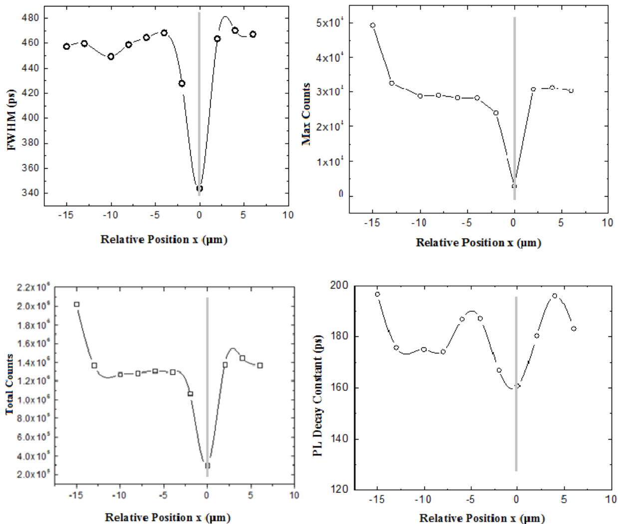
Figure 22: FWHM, maximum counts, total counts, and PL decay time constants from exponential fit of PL decay curves for eleven points along a straight line through the center of the extended defect (center at x=0 , indicated by vertical line) at 25% of maximum power. Note higher values of the decay constant \tau on either side of the defect.
