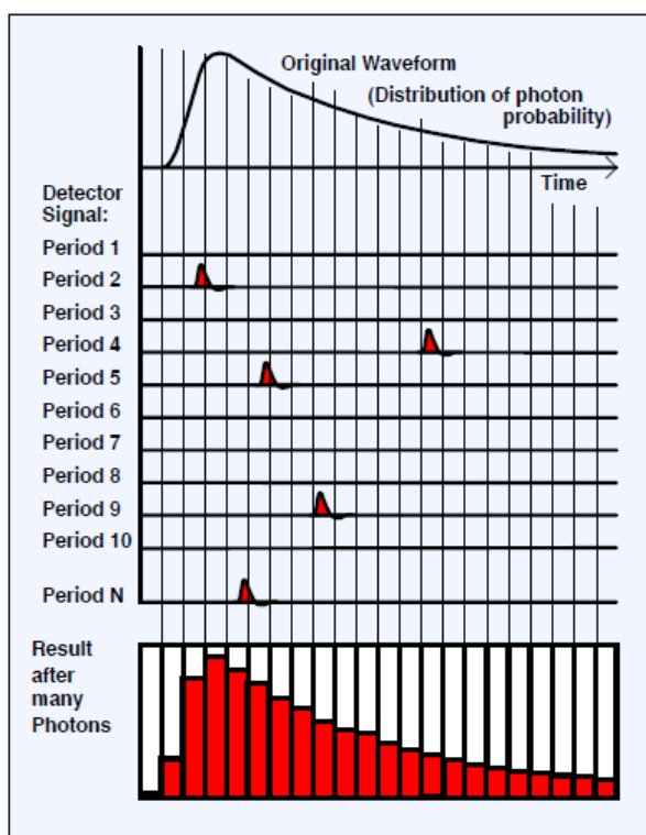
Figure 9: Principle of time correlated single photon counting. Individual photon counts accumulate in time channels which correspond to the arrival time of the pulse, thus creating a decay curve histogram (adapted from Becker and Hickl TCSPC Handbook, 6 th ed.)
