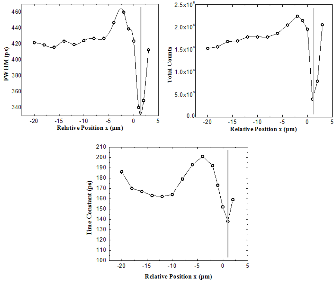
Figure 24: FWHM, total counts, and PL decay time constants vs. position for a linear scan from 20 \mu\text{m} from defect to just beyond defect center ( x=2\mu\text{m} ). Defect center is indicated by vertical line.
