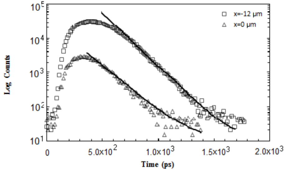
Figure 25: Semi-log plots of PL decay curves from figure 20 fit to eq. 10. Solid lines represent best nonlinear least squares fit using MATLAB™. Note lifetime in the defect is shown to be longer than at 12 μm distance.
