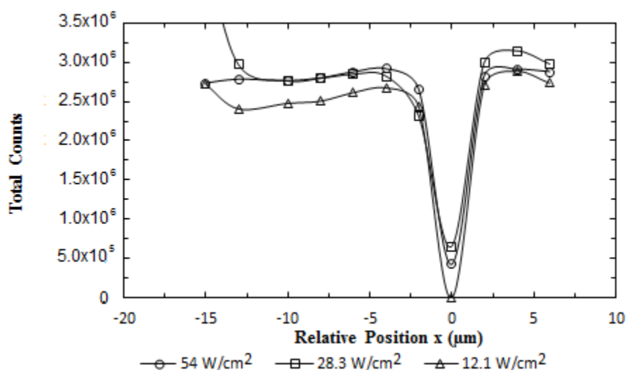
Figure 23: Plot of normalized total counts vs. position for three different excitation power levels (defect centers at x = 0 ).
