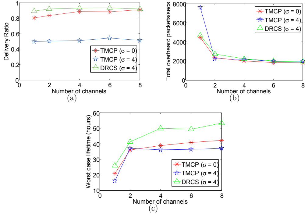
Figure 10.6: Comparison of (a) packet delivery ratio, (b) network-wide packets overheard (c) worst case network lifetime with different number of channels.
