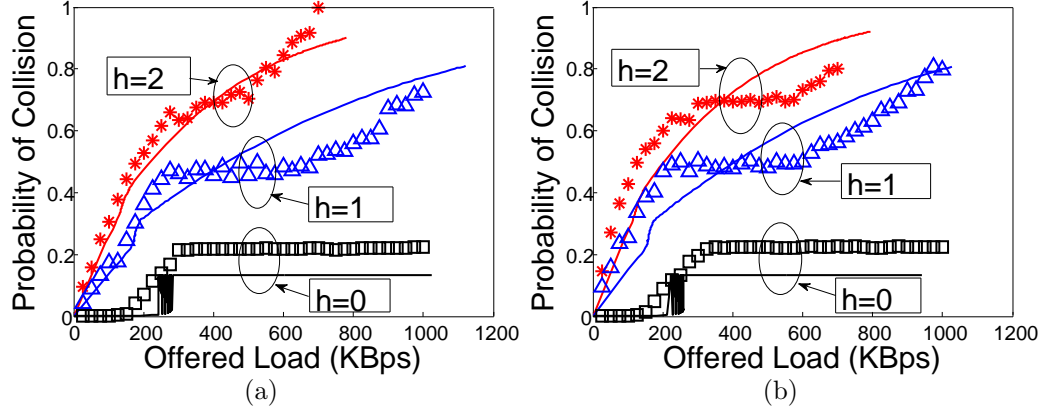
Figure 7.3: Probability of collision of contending stations with different offered load (a) Basic access mechanism, (b) RTS/CTS access mechanism.
