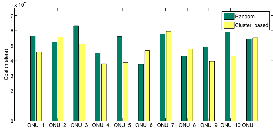
Figure 3.5: Costs of different ONUs for random placement and clustering-based schemes where mesh routers are uniformly distributed.
