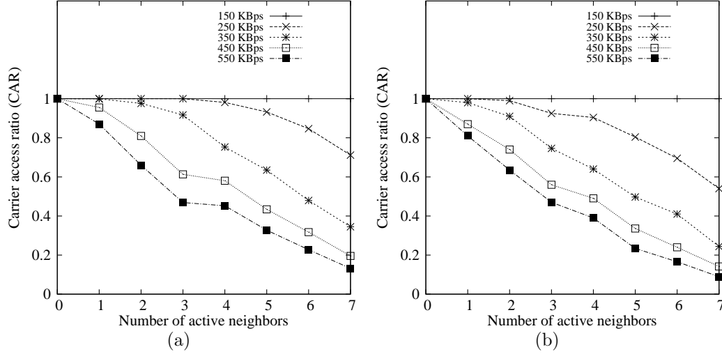
Figure 4.3: Variation of CAR (a) without RTS/CTS, (b) with RTS/CTS.
