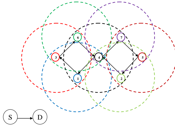
Figure A.1: Effect of dependent interferers on test link S \rightarrow D .
