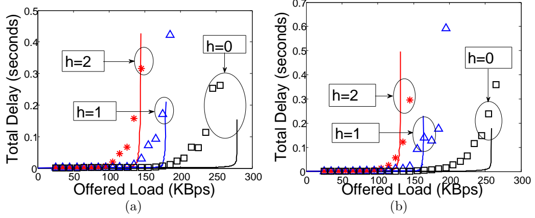
Figure 7.5: Total delay of contending stations with different offered load (a) Basic access mechanism, (b) RTS/CTS access mechanism.
