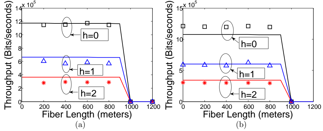
Figure 7.9: Individual throughput of contending stations with different fiber length (a) Basic access mechanism, (b) RTS/CTS access mechanism.
