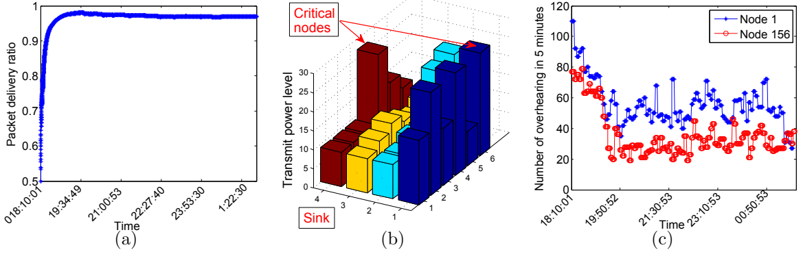
Figure 11.8: (a) Overall packet delivery ratio to the sink over time. (b) Transmit power levels of different nodes, power level 27 corresponds to -1 dBm and power level 9 corresponds to -13.4 dBm. (c) Number of packets overheard by the two critical nodes over time.
