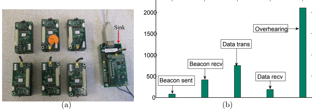
Figure 8.2: Experimental setup (a) to assess the activities of the radio (b) of a wireless sensor node performing data collection.
