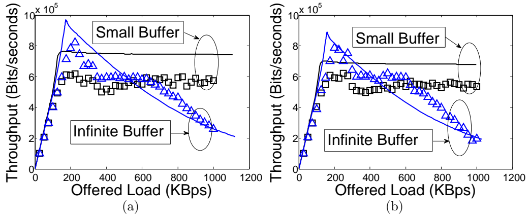
Figure 7.6: Individual throughput of contending stations with different offered load (a) Basic access mechanism, (b) RTS/CTS access mechanism.
