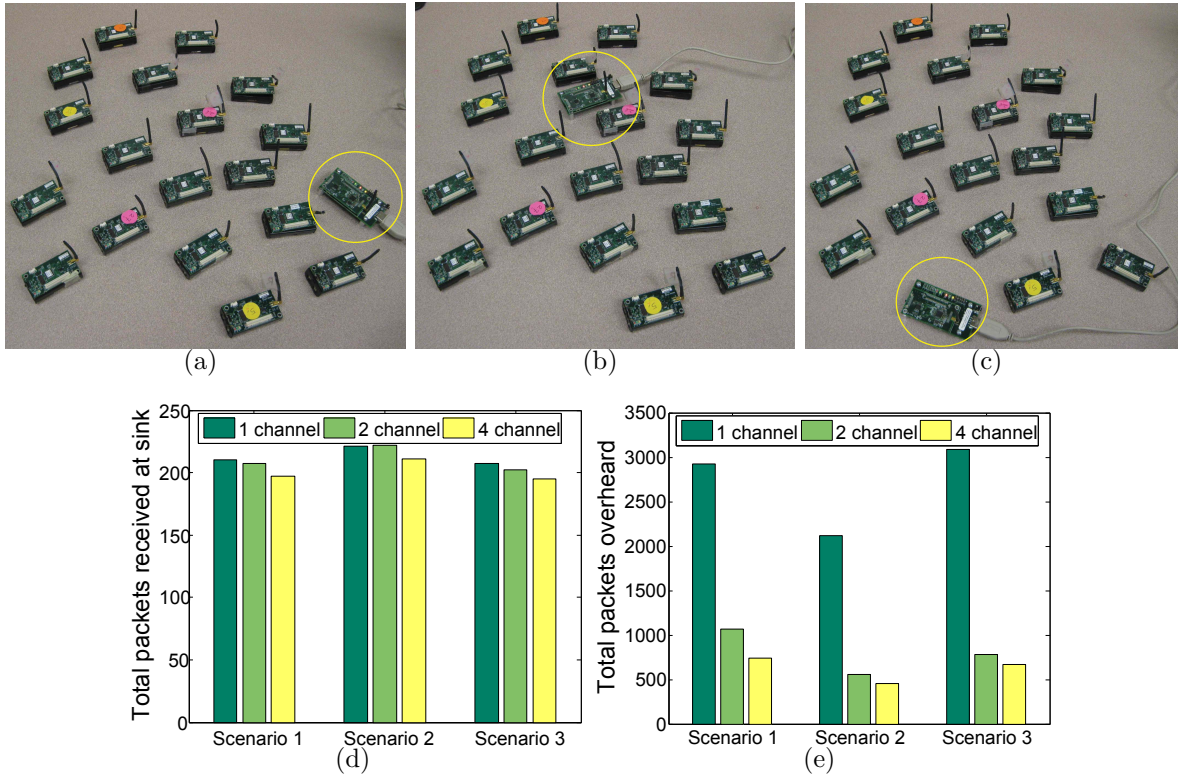
Figure 10.3: Experimental deployment scenarios with sink locations marked by yellow circles: 1 (a), 2 (b), and 3 (c); and comparison of the number of packets delivered at the sink (d) and the total packets overheard (e), with 1, 2, and 4 channels.
