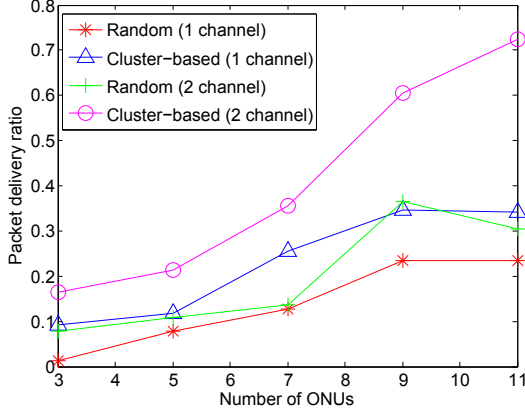
Figure 3.6: Comparison of delivery ratio with different number of ONUs for random placement and clustering-based schemes for uniform distribution of mesh routers.
