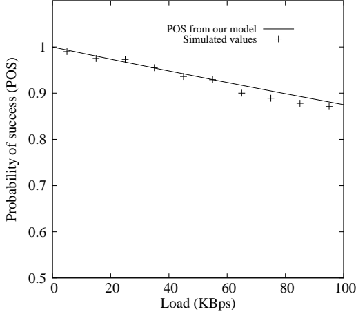
Figure 4.6: Experimentally obtained POS versus load in presence of 1 interferer.
