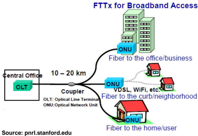
Figure 2.1: A PON architecture for optical access.
