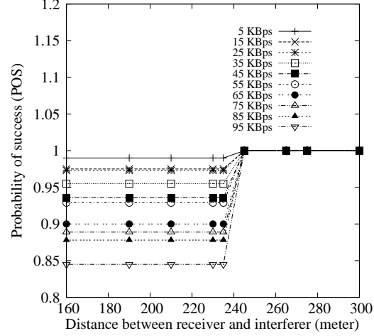
Figure 4.5: Variation of POS with respect to distance from an interferer.
