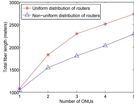
Figure 3.15: Comparison of total fiber length required for tree PON architecture for uniform and non-uniform distribution of mesh routers.
