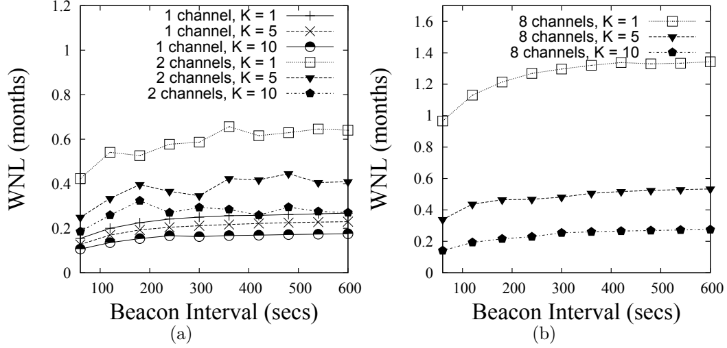
Figure 9.7: Comparison of lifetime when initial battery capacities are uniformly distributed for (a) DRCA-3, 1 and 2 channels (b) 8 channels.
