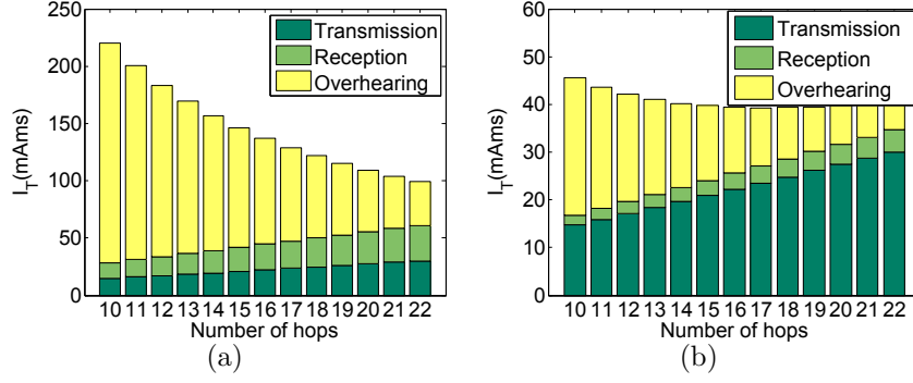
Figure 12.3: Variation of I_T with K when D = 200 meters and \rho = 0.0125 nodes/meters 2 for MICA2 motes (a) with typical value of I_r = 10 mA, and (b) with a fictitious value of I_r = 1.5 mA.
