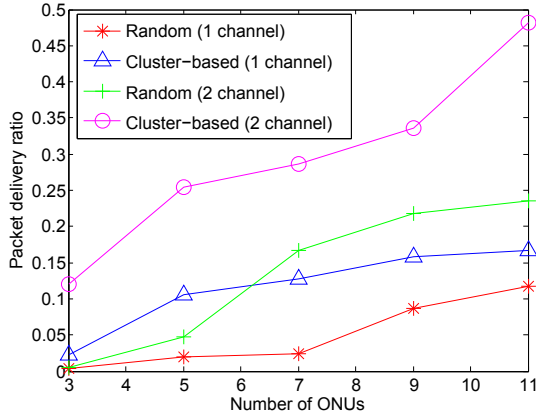
Figure 3.11: Comparison of delivery ratio with different number of ONUs for random placement and clustering-based schemes for non-uniform distribution of mesh routers.
