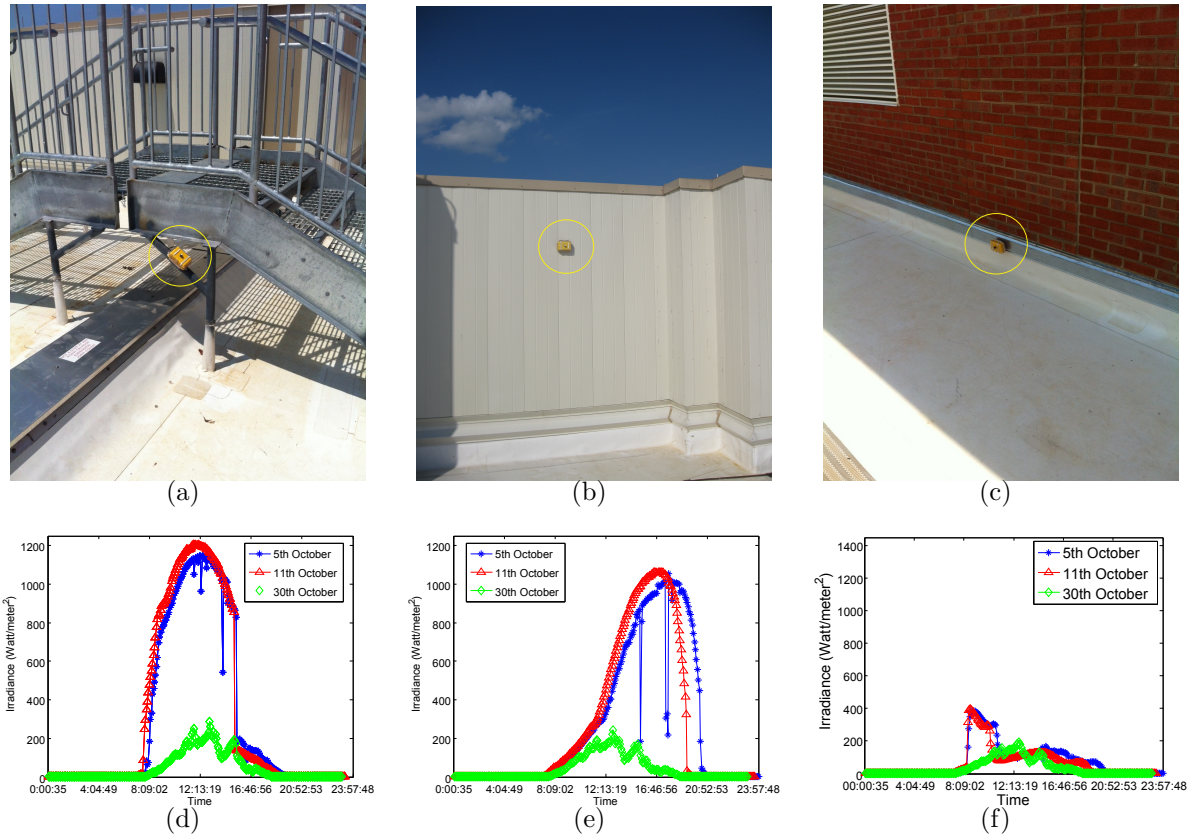
Figure 8.5: Samples of nodes deployed in EPIC-RoofNet (a) Node 153 (b) Node 155 (c) Node 159. Irradiance measurement of (d) node 153 (e) node 155 and (f) node 159 for two sunny days (5th and 11th October, 2012) and a cloudy day (30th October, 2012). Node 159 is kept in the shaded region, whereas 153 and 155 gets sunlight most of the time.
