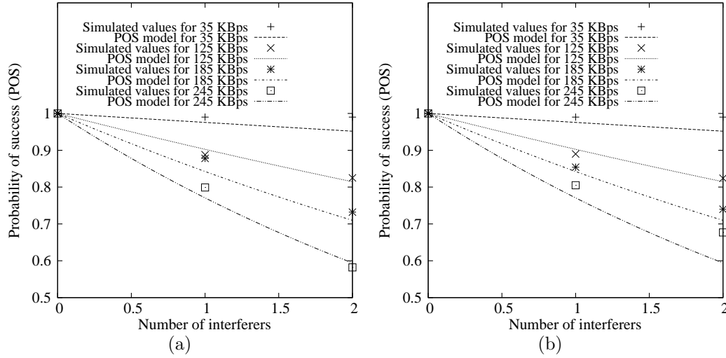
Figure 4.9: POS with (a) number of sending nodes among PC_i ( p ), (b) with number of receiving nodes among PC_i ( r ).
