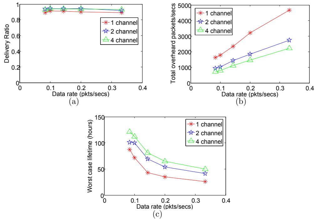
Figure 10.5: Comparison of (a) packet delivery ratio (b) network-wide packets overheard (c) worst case network lifetime with different data rates.
