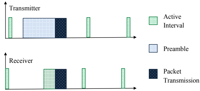
Figure 8.1: Low power listening.
