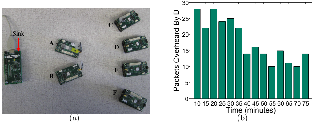
Figure 10.4: Experiment to evaluate the effectiveness of dynamic transmit channel selection.
