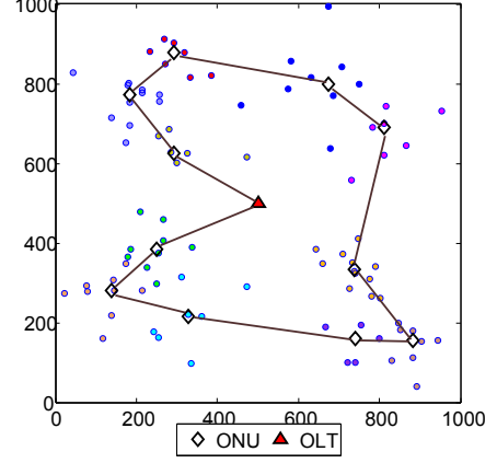
Figure 3.17: Fiber layout by solving the travelling salesman problem for non-uniform distribution of mesh routers.
