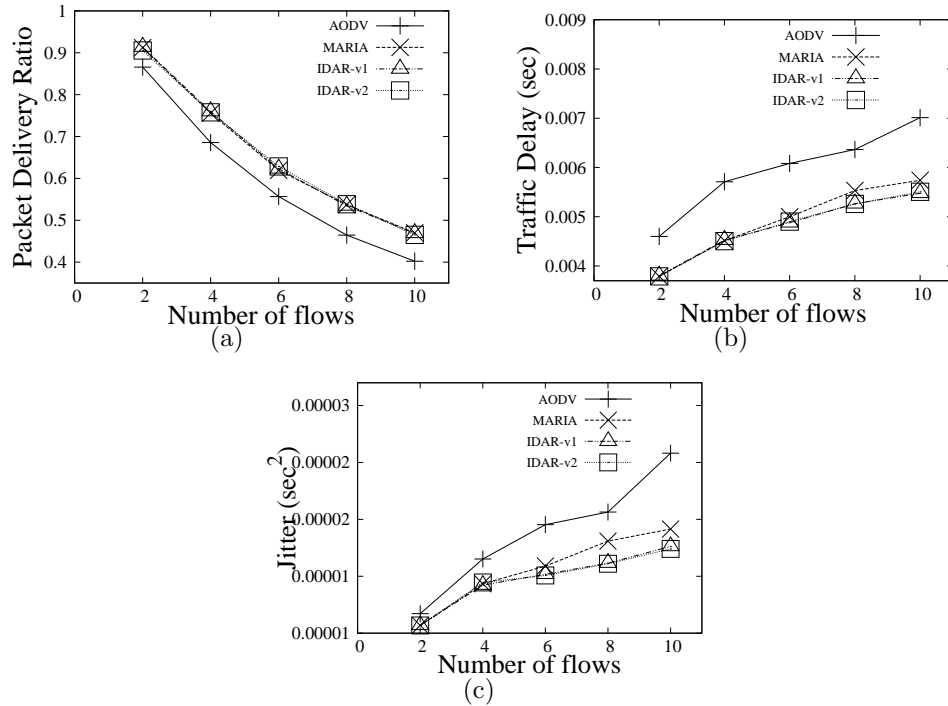
Figure 4.11: Comparison of (a) packet delivery ratio (b) delay (c) jitter
