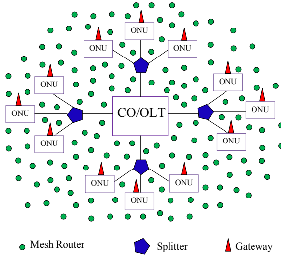
Figure 2.3: Architecture of a WOBAN.
