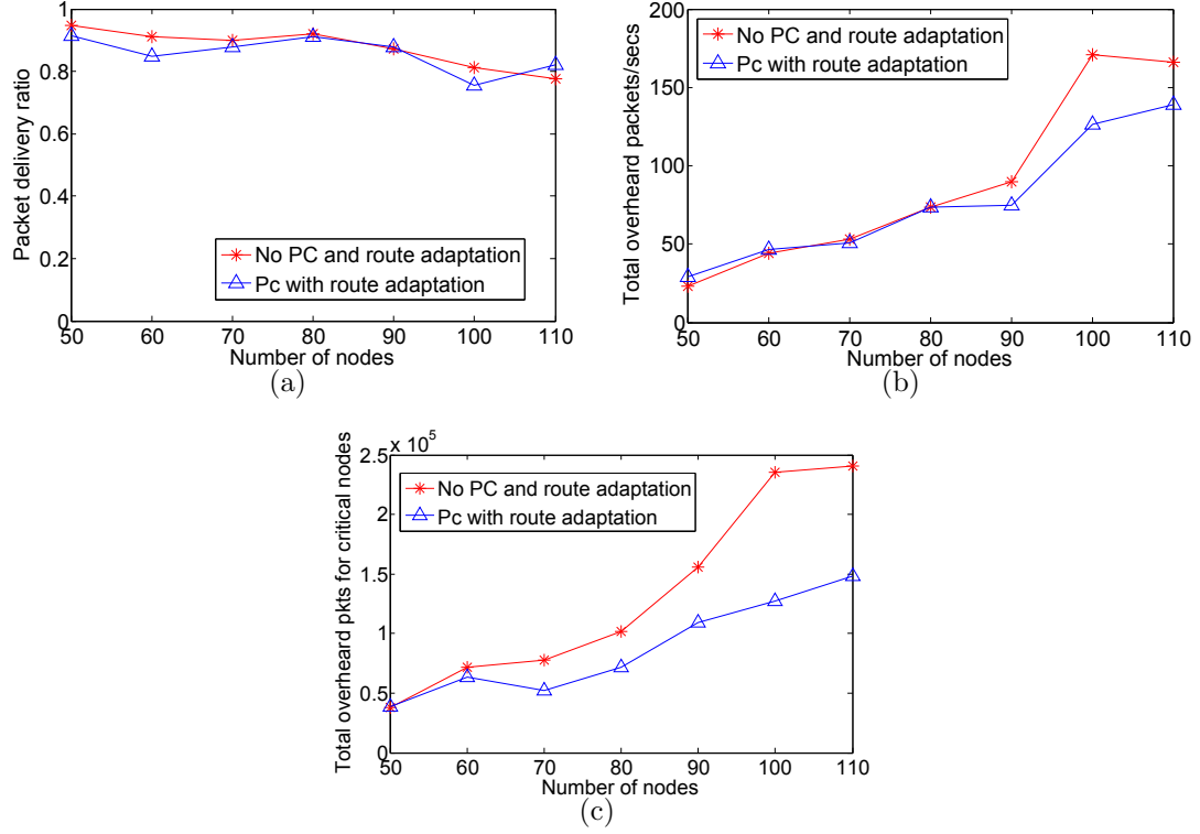
Figure 11.5: Comparison of (a) packet delivery ratio (b) network-wide packets overheard (c) packets overheard by the critical nodes with different node density.
