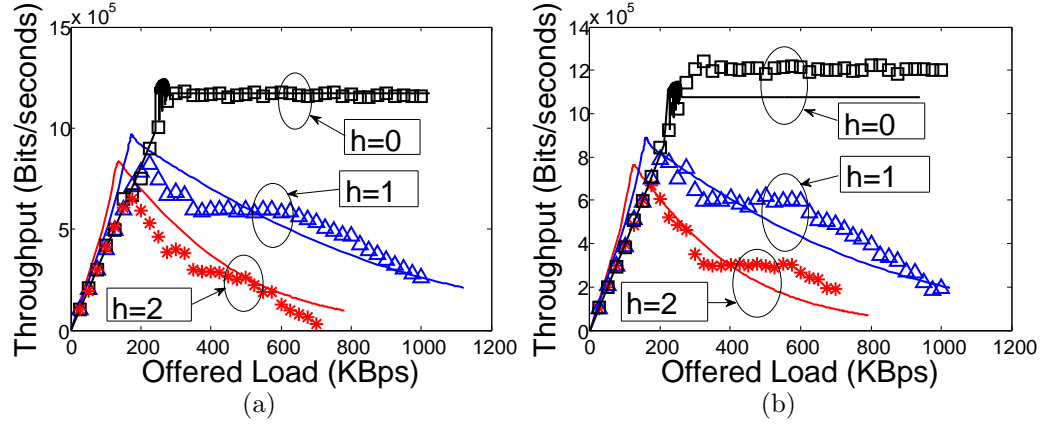
Figure 7.2: Individual throughput of contending stations with different offered load (a) Basic access mechanism, (b) RTS/CTS access mechanism.
