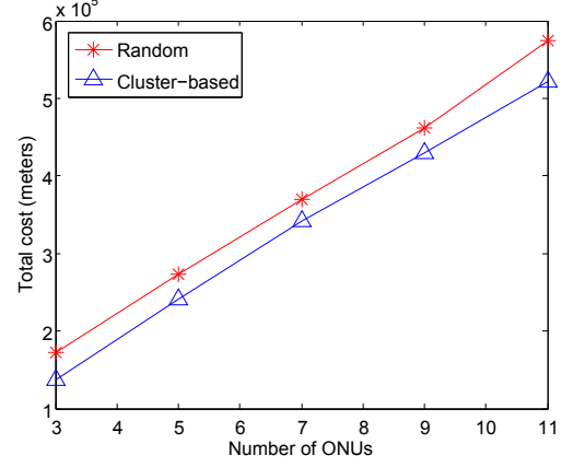
Figure 3.4: Comparison of overall cost for random placement and clustering-based schemes for uniform distribution of mesh routers.
