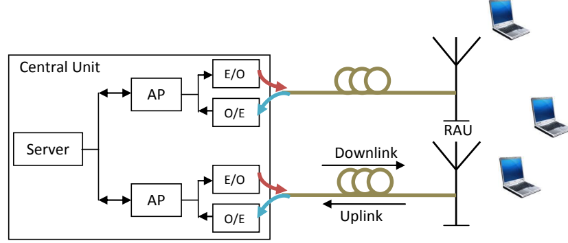
Figure 7.1: Block diagram of a radio-over-fiber network.
