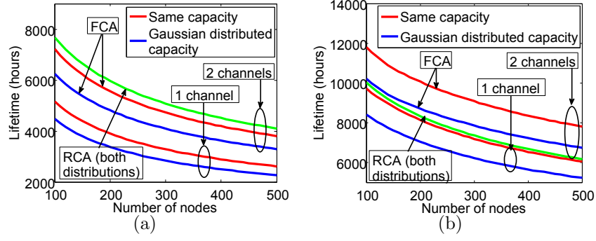
Figure 12.6: Expected network lifetime with different number of nodes (a) \alpha_r = 10 mA and (b) \alpha_r = 1.5 mA.
