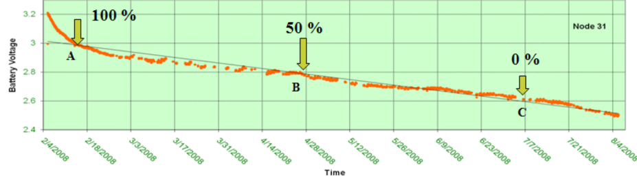
Figure 10.1: Battery discharge curve of a typical node in Paradisenet .
