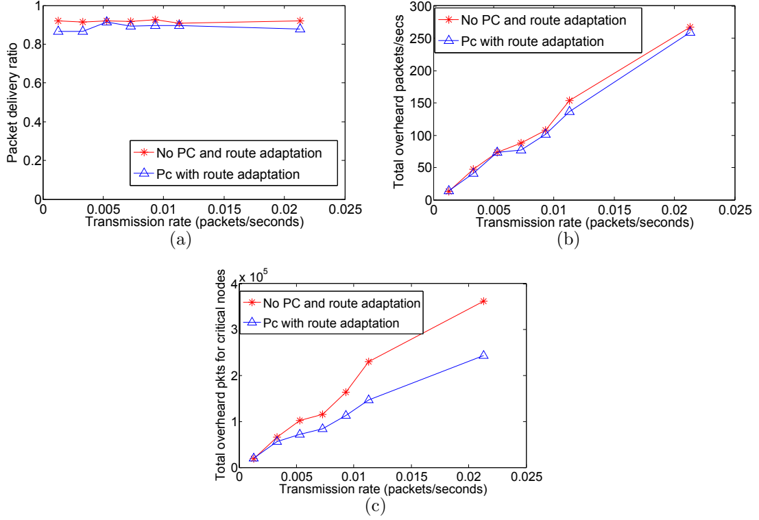
Figure 11.4: Comparison of (a) packet delivery ratio (b) network-wide packets overheard (c) packets overheard by the critical nodes with different rates.
