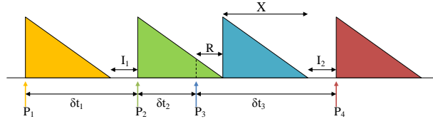
Figure A.2: Interarrival time ( \delta t ), residual time ( R ), service time ( \bar{X} ) and Idle periods ( I ) of a queuing system.
