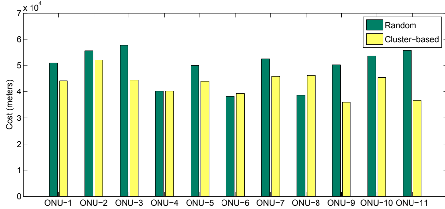
Figure 3.10: Costs of different ONUs for random placement and clustering-based schemes where mesh routers are non-uniformly distributed.
