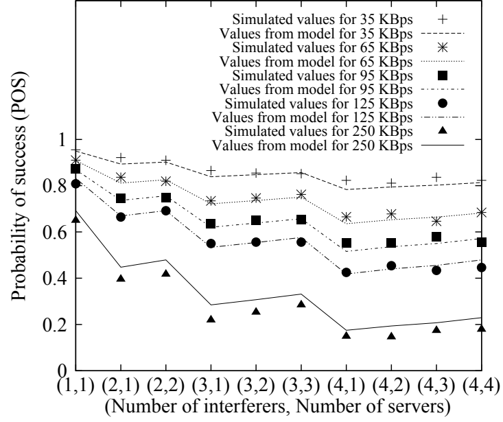
Figure A.4: POS in presence of dependent interferers around D: model and simulation results.
