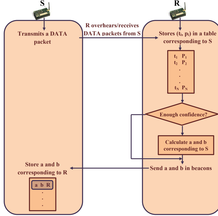
Figure 11.2: Receiver-oriented prediction model.
