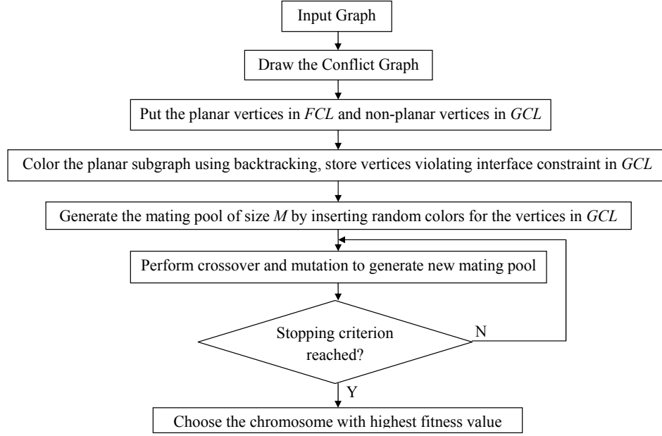
Figure 6.4: Joint route and channel assignment (JRCA) scheme.
