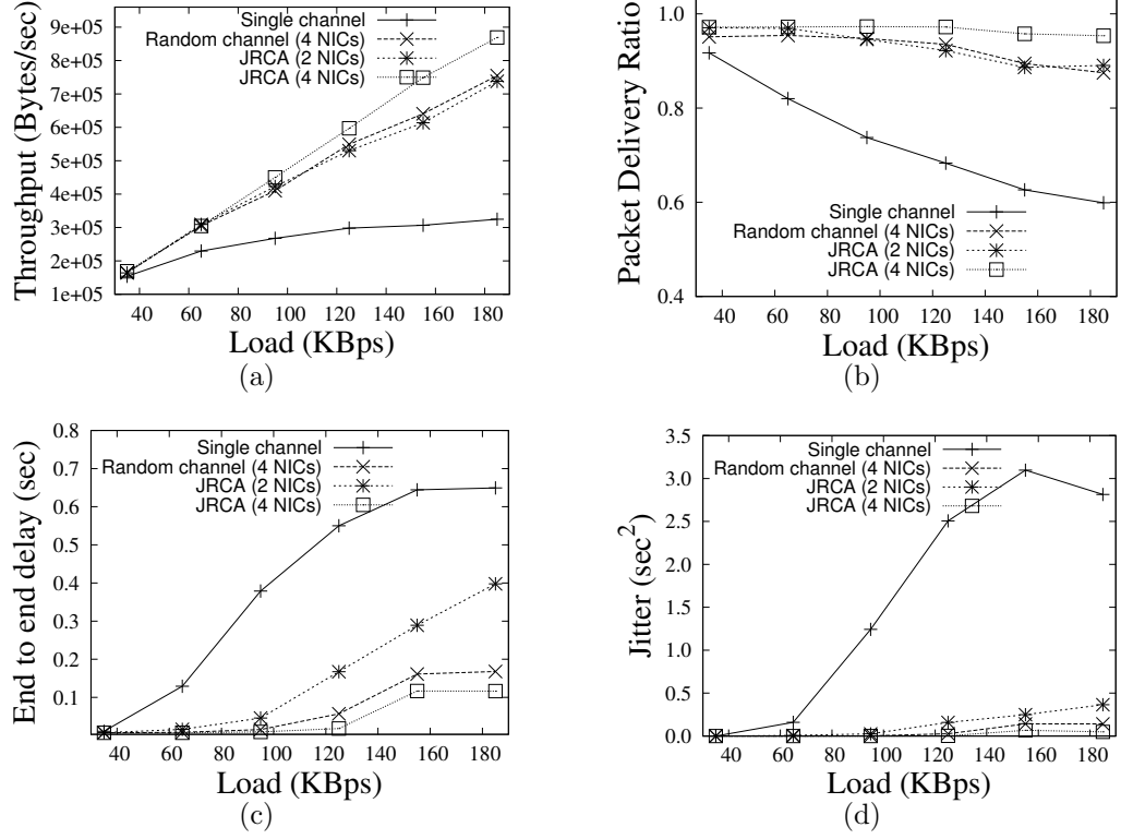
Figure 6.6: Comparison of (a) throughput (b) delivery ratio (c) delay (d) jitter with different loads.
