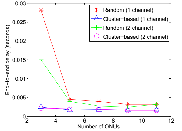
Figure 3.12: Comparison of end-to-end delay with different number of ONUs for random placement and clustering-based schemes for non-uniform distribution of mesh routers.
