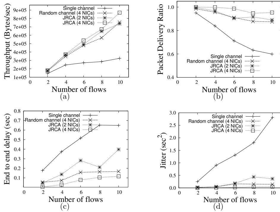
Figure 6.5: Comparison of (a) throughput (b) delivery ratio (c) delay (d) jitter with different number of flows.
