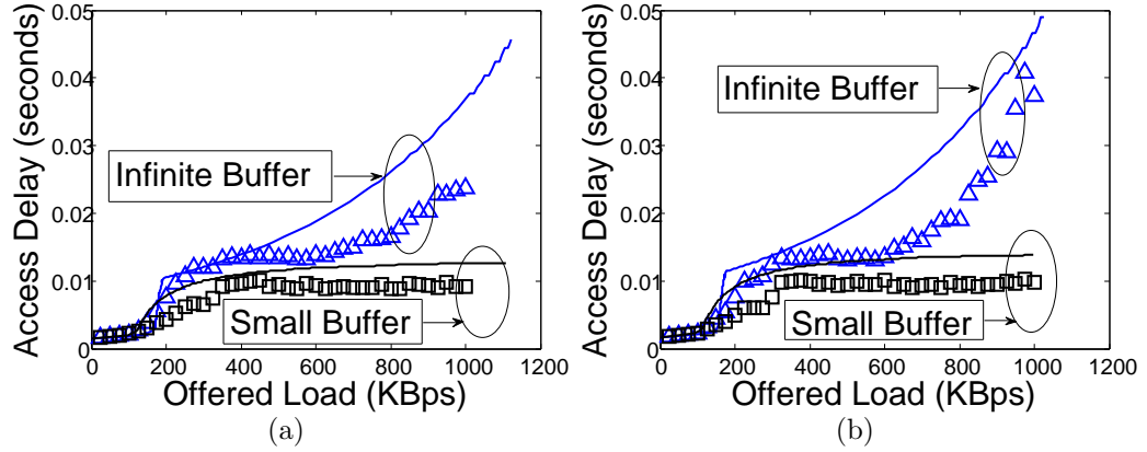
Figure 7.8: Access Delay of contending stations with different offered load (a) Basic access mechanism, (b) RTS/CTS access mechanism.
