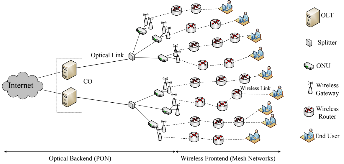
Figure 1.2: A typical WOBAN architecture.
