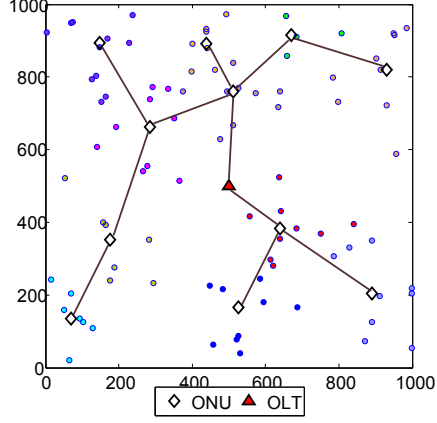
Figure 3.13: Fiber layout using minimum spanning tree for uniform distribution of mesh routers.
