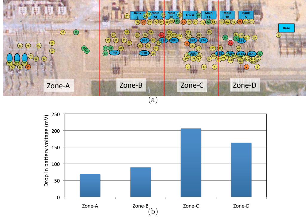
Figure 8.3: Illustration of the layout (a) of ParadiseNet [?], a 122-node WSN deployed for equipment health monitoring from a power substation, and the average battery usage of nodes in different geographical zones over a period of five months (b). ParadiseNet uses a single-channel link quality based routing protocol.
