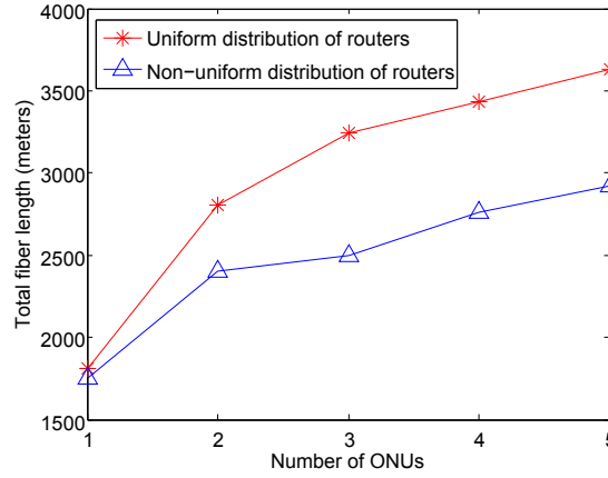
Figure 3.18: Comparison of total fiber length required for ring PON architecture for uniform and non-uniform distribution of mesh routers.
