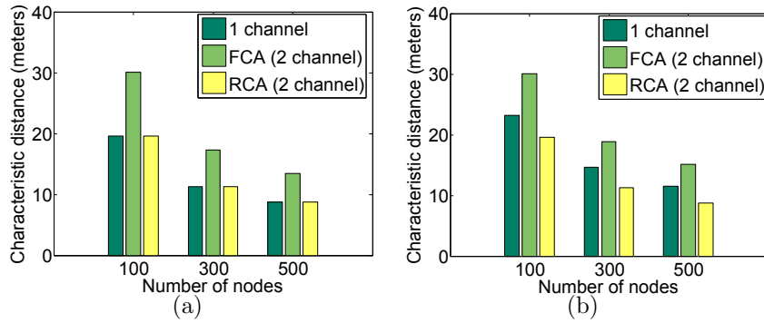
Figure 12.5: Characteristic distance with different number of nodes (a) \alpha_r = 10 mA and (b) \alpha_r = 1.5 mA.
