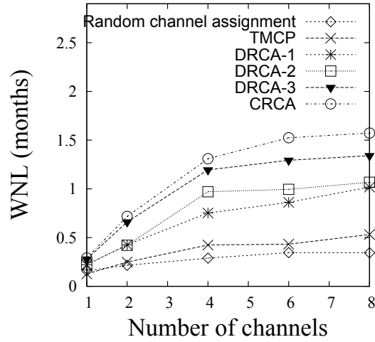
Figure 9.6: Comparison of lifetime when different number of channels.
