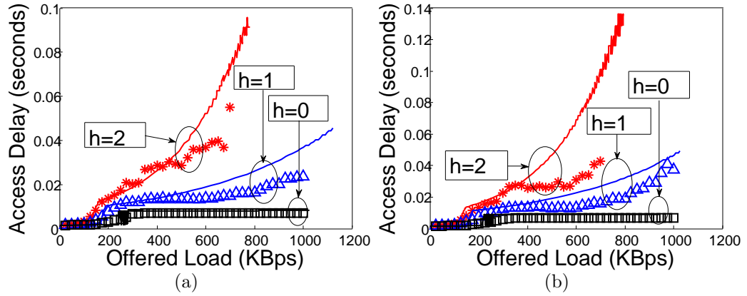
Figure 7.4: Access delay of contending stations with different offered load (a) Basic access mechanism, (b) RTS/CTS access mechanism.
