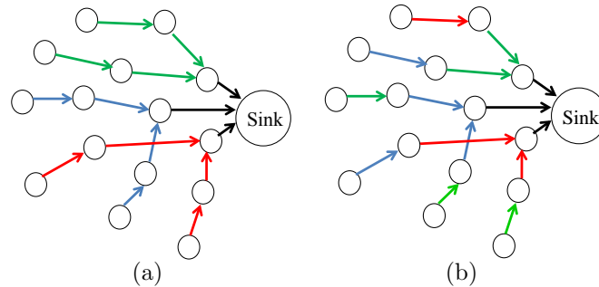
Figure 8.6: Channel assignment schemes (a) FCA, (b) RCA.
