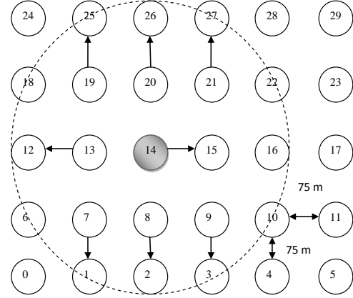
Figure 4.2: Simulation environment to evaluate the effect of active neighbors on the test link 14→15. The dotted line shows the carrier sensing range.
