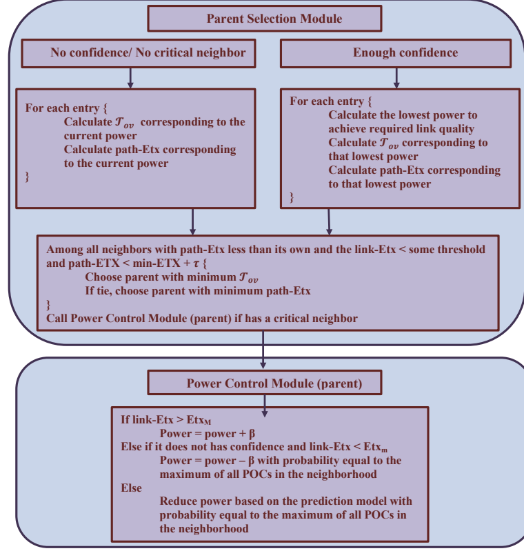
Figure 11.3: Proposed joint power control and route adaptation scheme.
