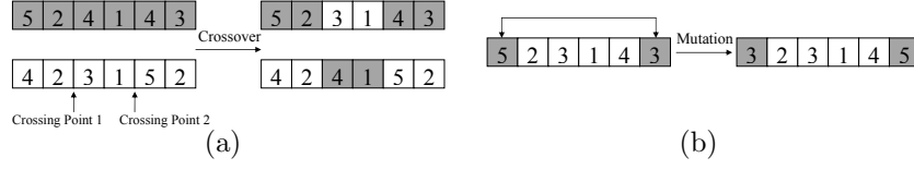
Figure 6.3: (a) Two-point crossover and (b) Mutation.
