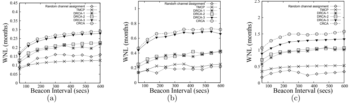
Figure 9.5: Comparison of lifetime when initial battery capacities are uniformly distributed for (a) 1 channel (b) 2 channels (c) 8 channels.
