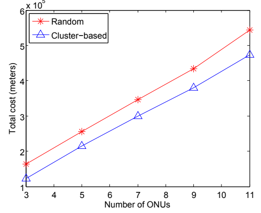
Figure 3.9: Comparison of overall cost for random placement and clustering-based schemes for non-uniform distribution of mesh routers.
