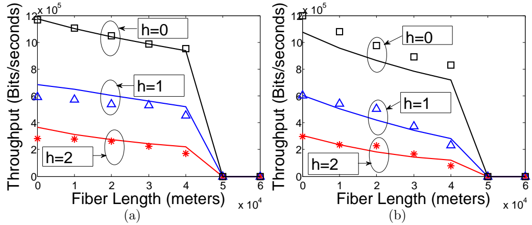
Figure 7.10: Individual throughput of contending stations with different fiber length (a) Basic access mechanism, (b) RTS/CTS access mechanism.
