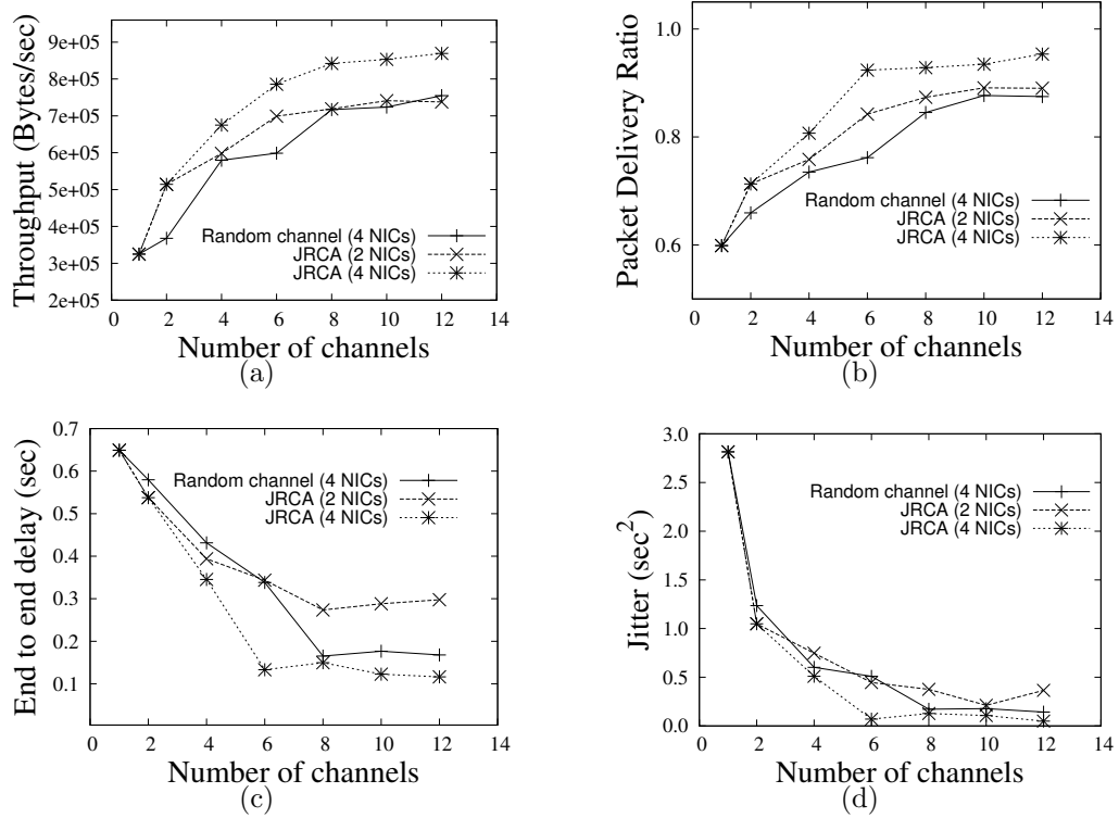
Figure 6.7: Comparison of (a) throughput (b) delivery ratio (c) delay (d) jitter with different number of channels.
