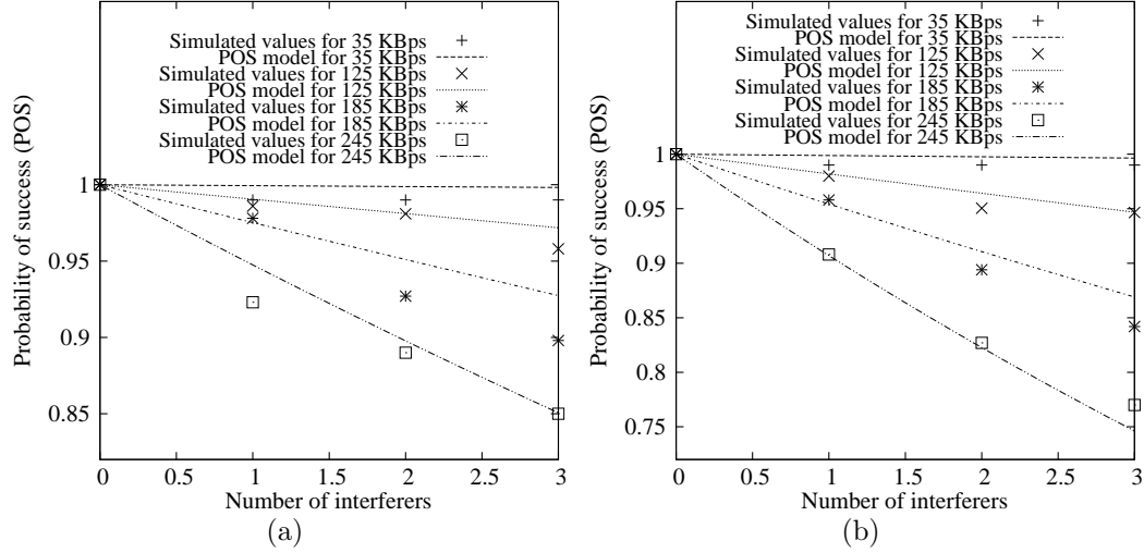
Figure 4.10: POS with number of active nodes among NC_i ( n ) (a) with m = 1 , (b) with m = 2 .
