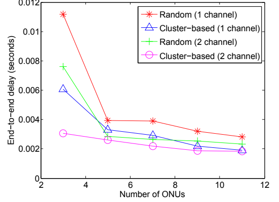
Figure 3.7: Comparison of end-to-end delay with different number of ONUs for random placement and clustering-based schemes for uniform distribution of mesh routers.
