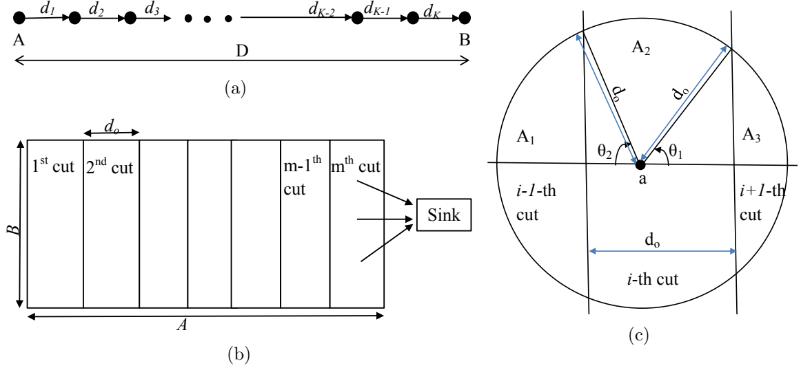
Figure 12.2: (a) Introducing K - 1 relay between A and B. (b) A sensor network with N nodes in a field of A \times B , (c) Calculating overhearing at the i -th cut.
