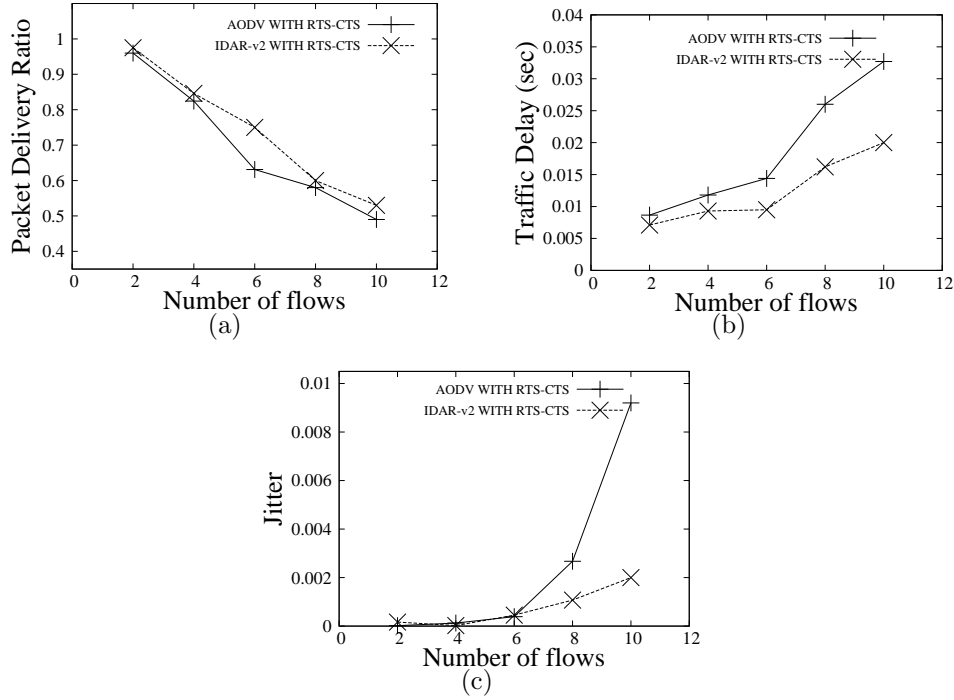
Figure 4.12: Comparison of (a) packet delivery ratio (b) delay (c) jitter
