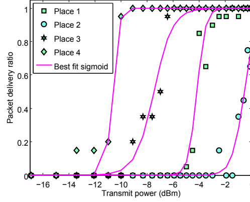
Figure 11.1: Sigmoid best fit curve of delivery ratio vs transmit power.
