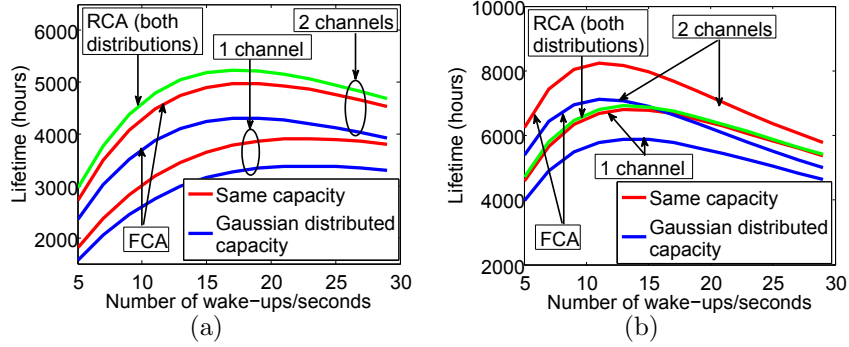
Figure 12.7: Expected network lifetime with different wake-up rates (a) \alpha_r = 10 mA and (b) \alpha_r = 1.5 mA.
