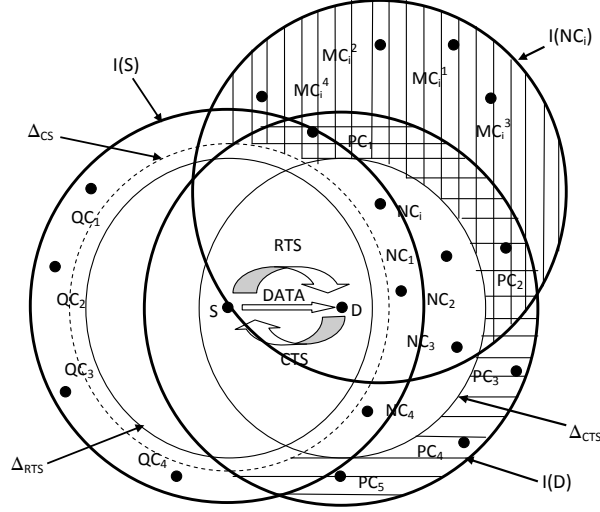
Figure 4.8: Effect of interferers in presence of RTS/CTS for test link S \rightarrow D
