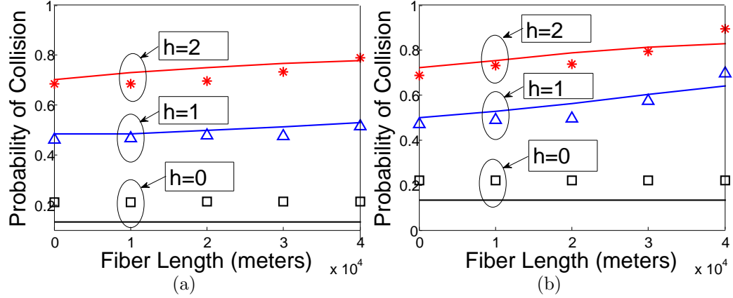
Figure 7.11: Probability of collision of contending stations with different fiber length (a) Basic access mechanism, (b) RTS/CTS access mechanism.
