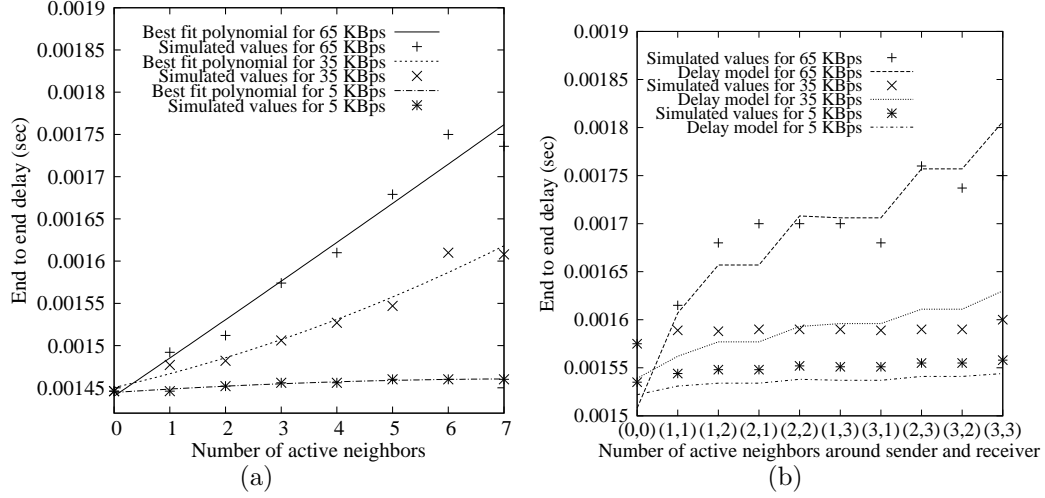
Figure 4.4: Variation of delay (a) with number of active neighbors of sender without RTS/CTS, (b) with number of active neighbors of sender and receiver with RTS/CTS.
