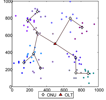
Figure 3.14: Fiber layout using minimum spanning tree for non-uniform distribution of mesh routers.
