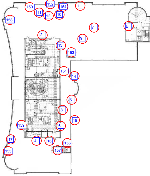
Figure 8.4: A MICAz wireless sensor network testbed EPIC-RoofNet .
