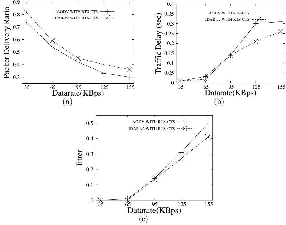
Figure 4.13: Comparison of (a) packet delivery ratio (b) delay (c) jitter
