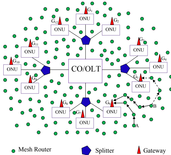
Figure 5.1: WOBAN with multiple gateways.
