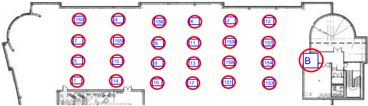
Figure 11.7: The map of the wireless sensor network testbed. Node 1 and Node 156 are made to be resource critical nodes.
