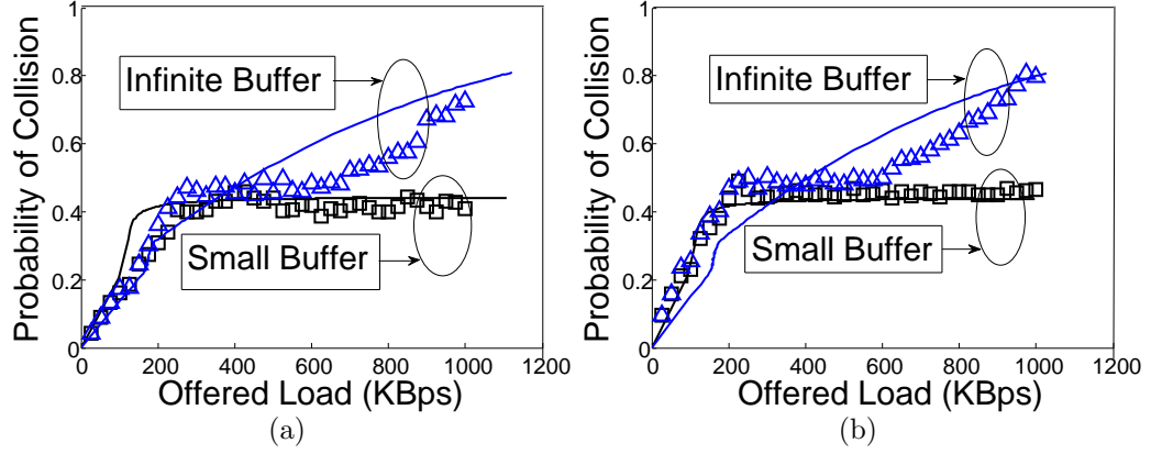
Figure 7.7: Probability of Collision of contending stations with different offered load (a) Basic access mechanism, (b) RTS/CTS access mechanism.
