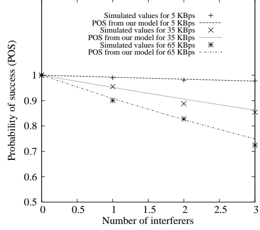
Figure 4.7: POS versus number of interferers of D : model and simulation results
