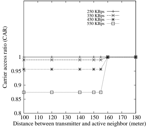
Figure 4.1: Variation of CAR with respect to distance from an active neighbor.
