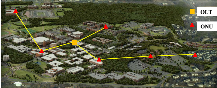
Figure 3.1: A hypothetical example of a WOBAN architecture in a campus network (UNC Charlotte campus).
